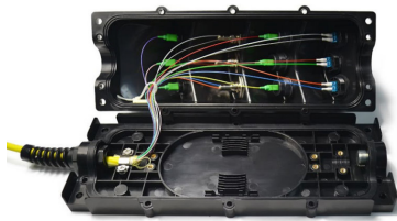
FTTX Enclosure w/ PLC Connection Project
